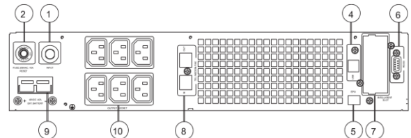
b. 0.9PF 1.5K&2KVA RT rear panel
