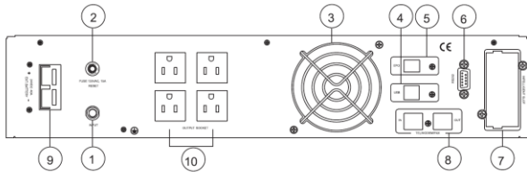
a. 0.9PF 1KVA RT rear panel
