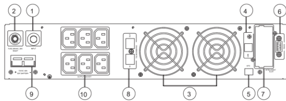
c. 0.9PF 3KVA RT rear panel
