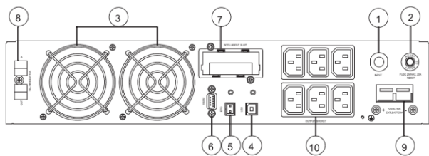
c. 0.9PF 3KVA RT rear panel
