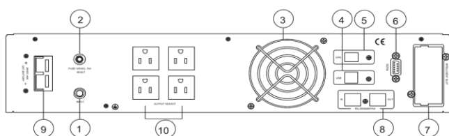
a. 0.9PF 1KVA RT rear panel
