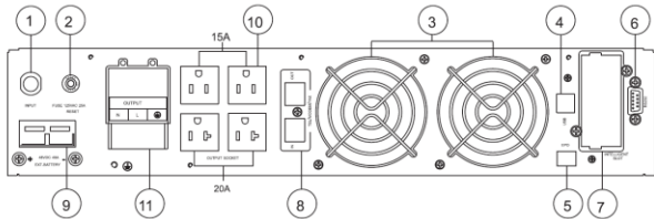
c. 0.9PF 3KVA RT rear panel
