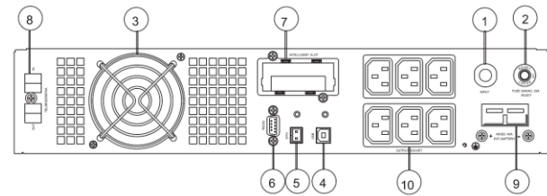
b. 0.9PF 1.5K&2KVA RT rear panel
