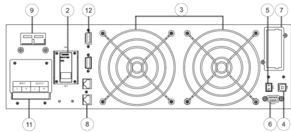
d. 0.9PF 6/10KVA RT rear panel
