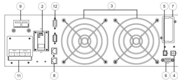
d. 0.9PF 6/10KVA RT rear panel
