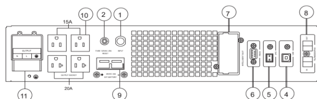
b. 0.9PF 1.5K&2KVA&3KVA RT rear panel
